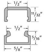
INF-X-CHAN-8 X = C (clear), F (frosted) PC extrusion, available in 8' lengths
